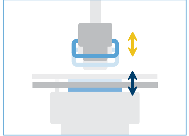
Motorized two-way vertical syncing of x-ray tube and table top, keeping preset source-image distance (SID) constant
