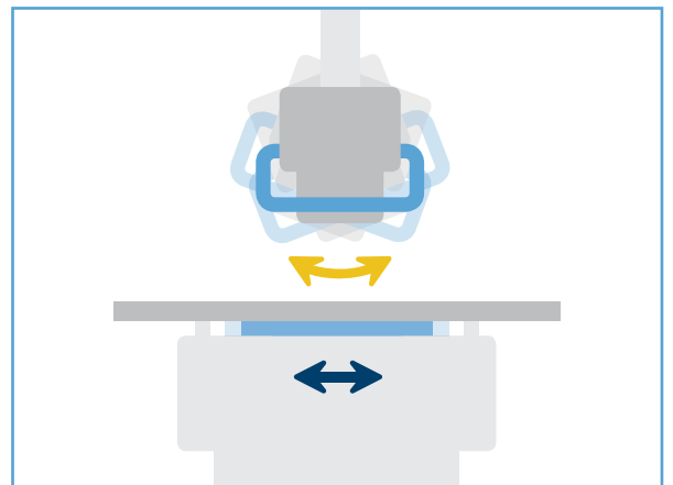
Motorized alignment of table image receptor with x-ray tube movement and rotation
